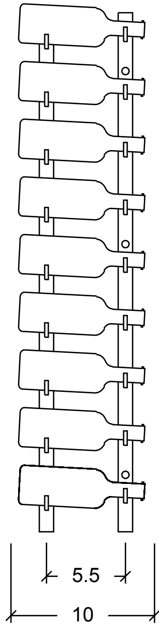
(Mounting for Splits) Front View
