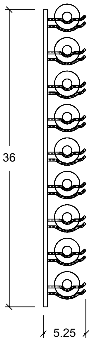
(Standard Mounting) Side View
