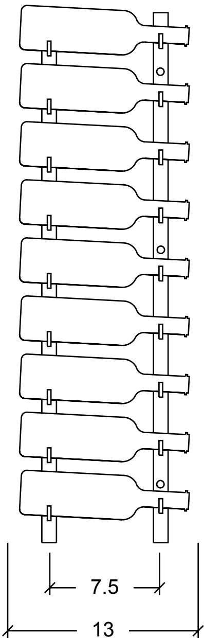
(Standard Mounting) Front View
