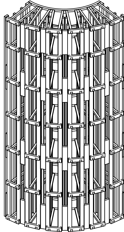
Back View
